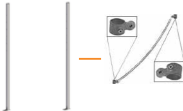
43756001 Leg 1500 mm 43756100 Leg 2200 mm 43757001 Stay-tube for legs >2200 mm
